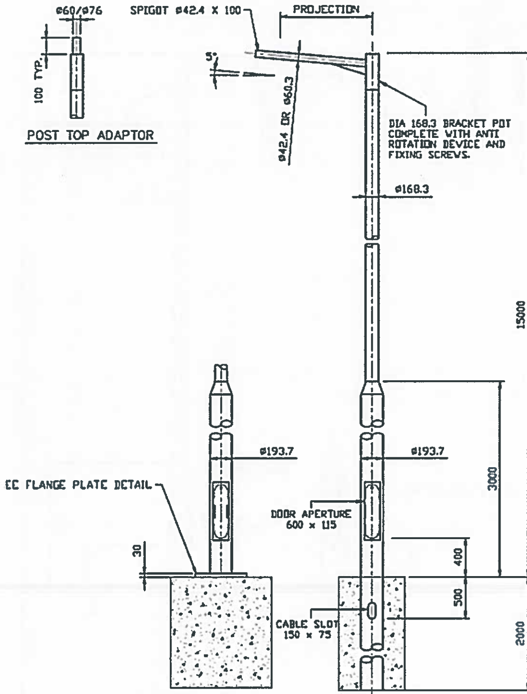
Fig. 1c. 15m Tubular Column Rooted and Flange Plated complete with various bracket arrangements
